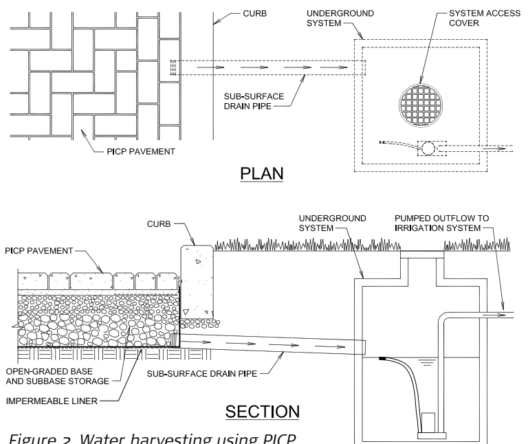
Figure 2. Water harvesting using PICP.
